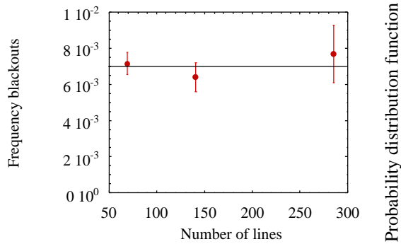
Fig. 9. Frequency of blackouts for the three tree networks listed in Table I.
