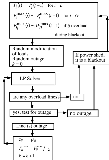
Fig. 1. Flow diagram of the implementation of the power transmission blackout model.
